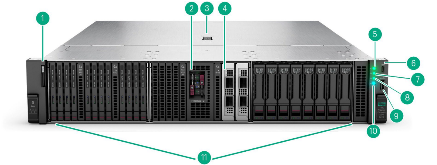
Front View - SFF/EDSFF CTO Server
