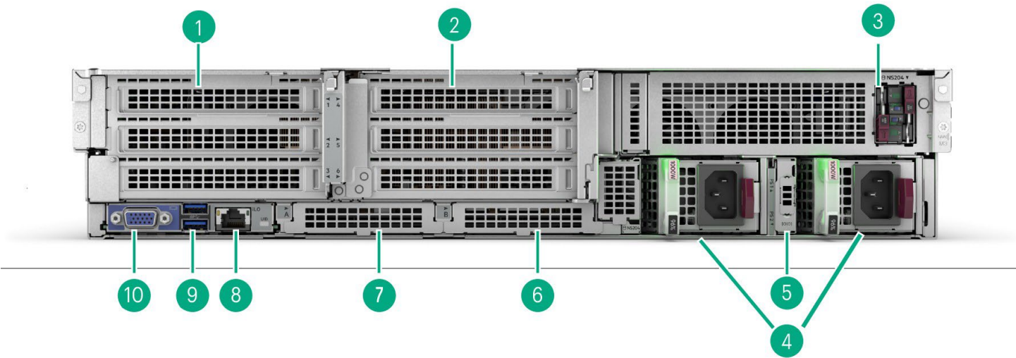
Rear View
