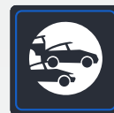
Vehicle Search
