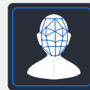
Face Detection
