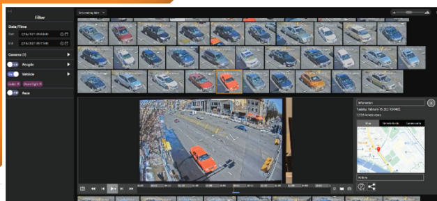
Vehicle Search
