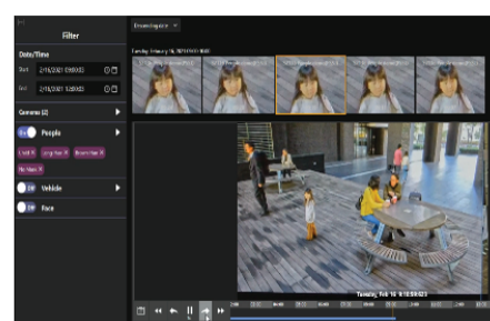
Face Search
