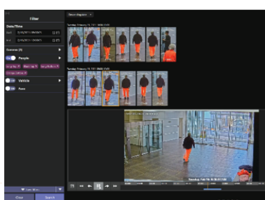
People Search
